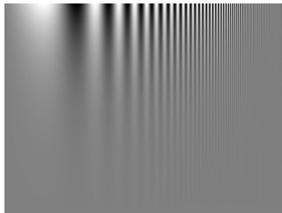
Figure 6: Contrast-Sensitivity Grating
